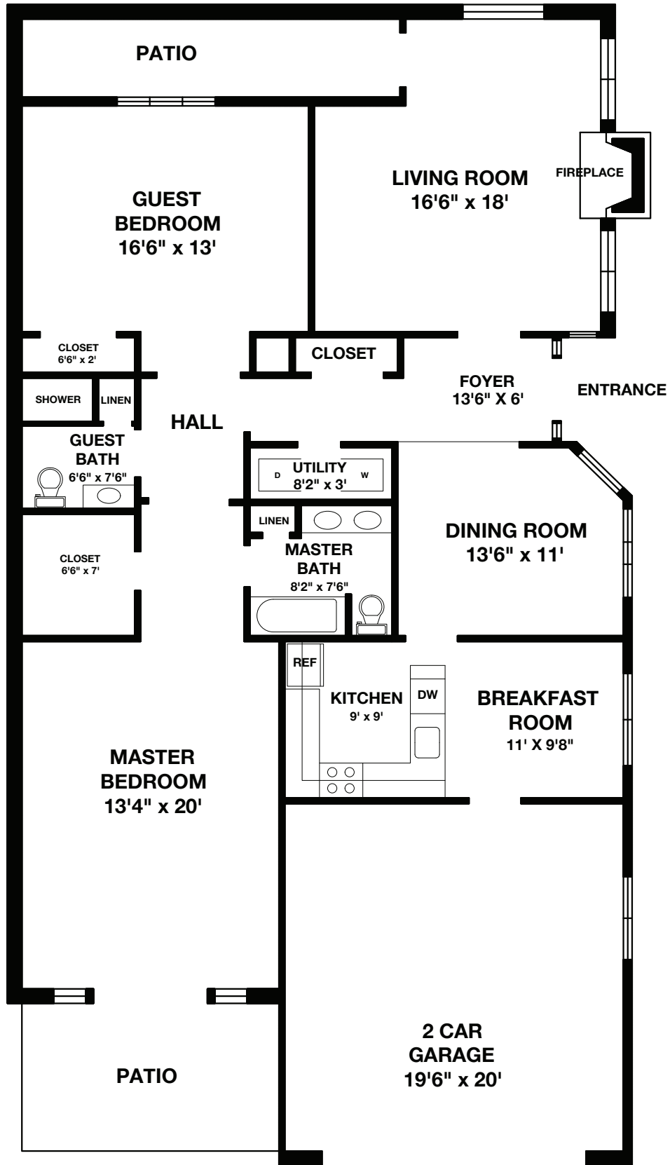
STYLE V2 One Level, Two Bedroom Villa Two Car Garage 1,578 Sq. Ft.
